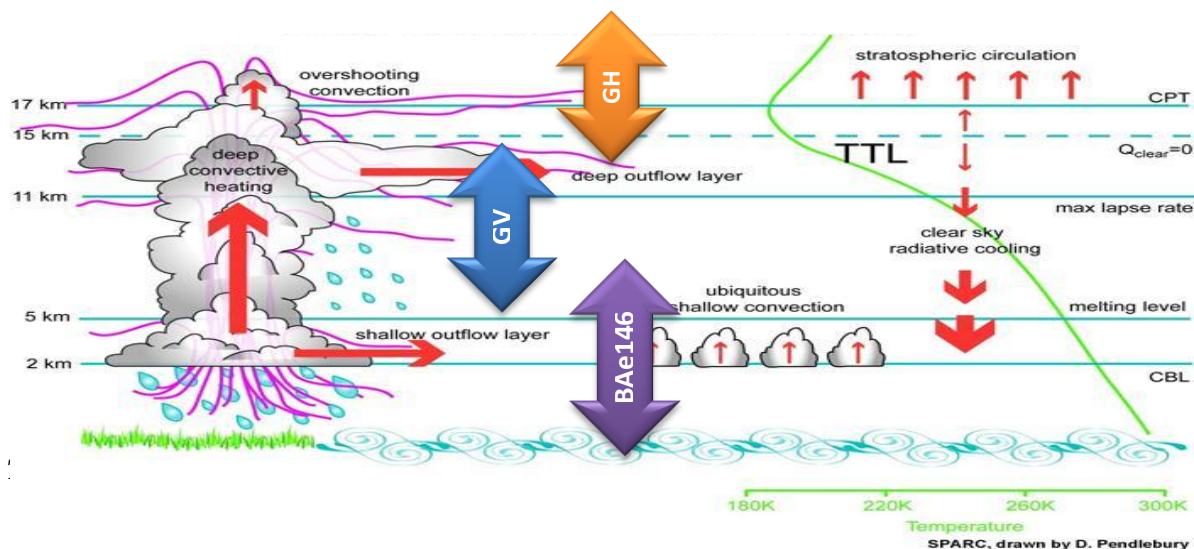
Figure 1. Schematic showing the convective processes in relation to the TTL, and typical altitude regions sampled by the CONTRAST GV, the ATTREX Global Hawk (GH), and CAST BAe-146 aircraft.
