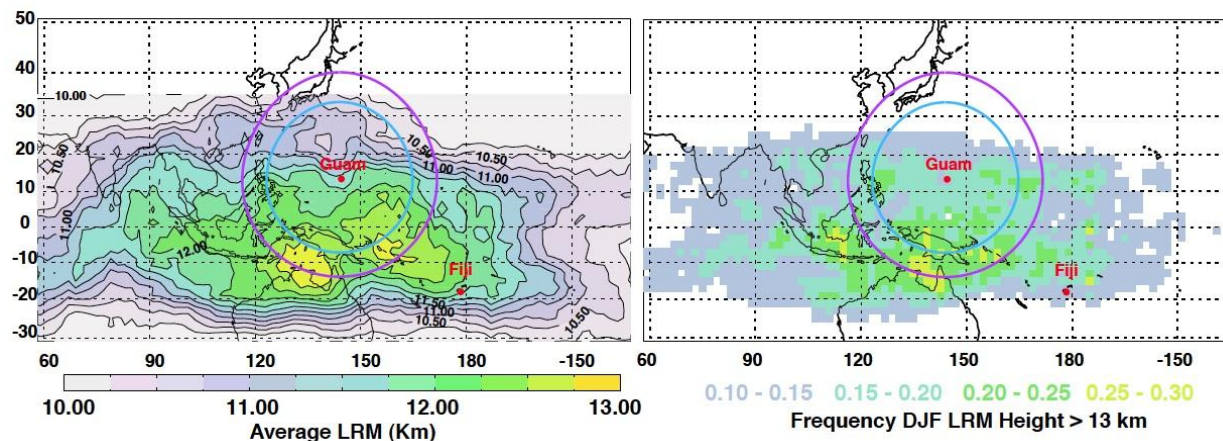
Figure 6. (left) Seasonal average of LRM based on four-year COSMIC GPS satellite temperature profiles. Calculation is done in 2x2 degree Lat/Lon bins. The highest average shown is 13 km. (Right) Frequency of occurrence of LRM greater than 13 km. The GV range is shown by the blue and purple rings.
